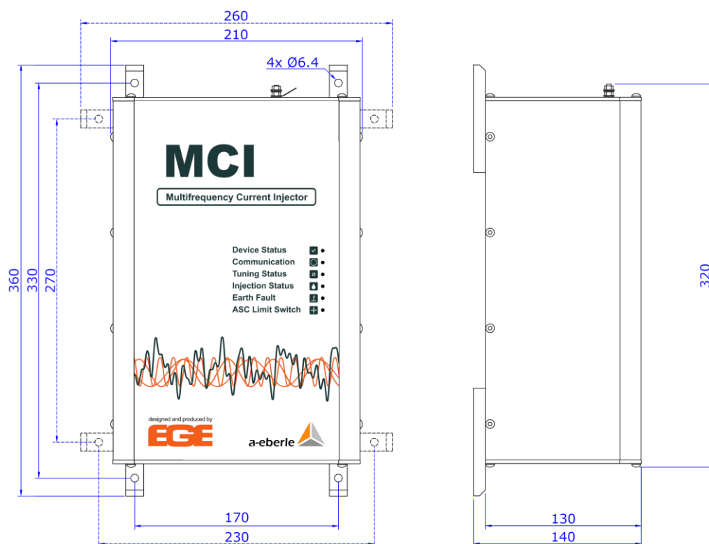
Figure 2: Basic MCI dimensions and layout of mounting holes
