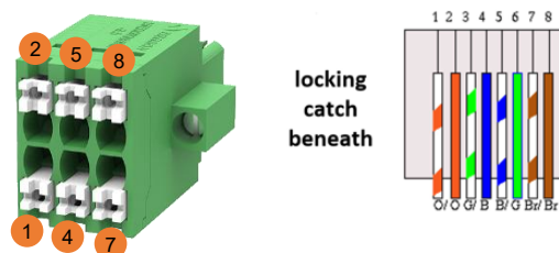
Figure 3: Communication connector for HW version >1.1 – left; RJ45 for HW version 1.0 (up to 2026) – right
