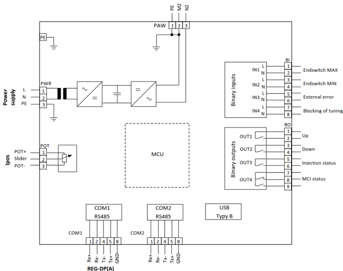
Figure 1: Block diagram of MCI
